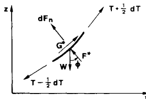
Fig. 2 Forces acting on cable element.
